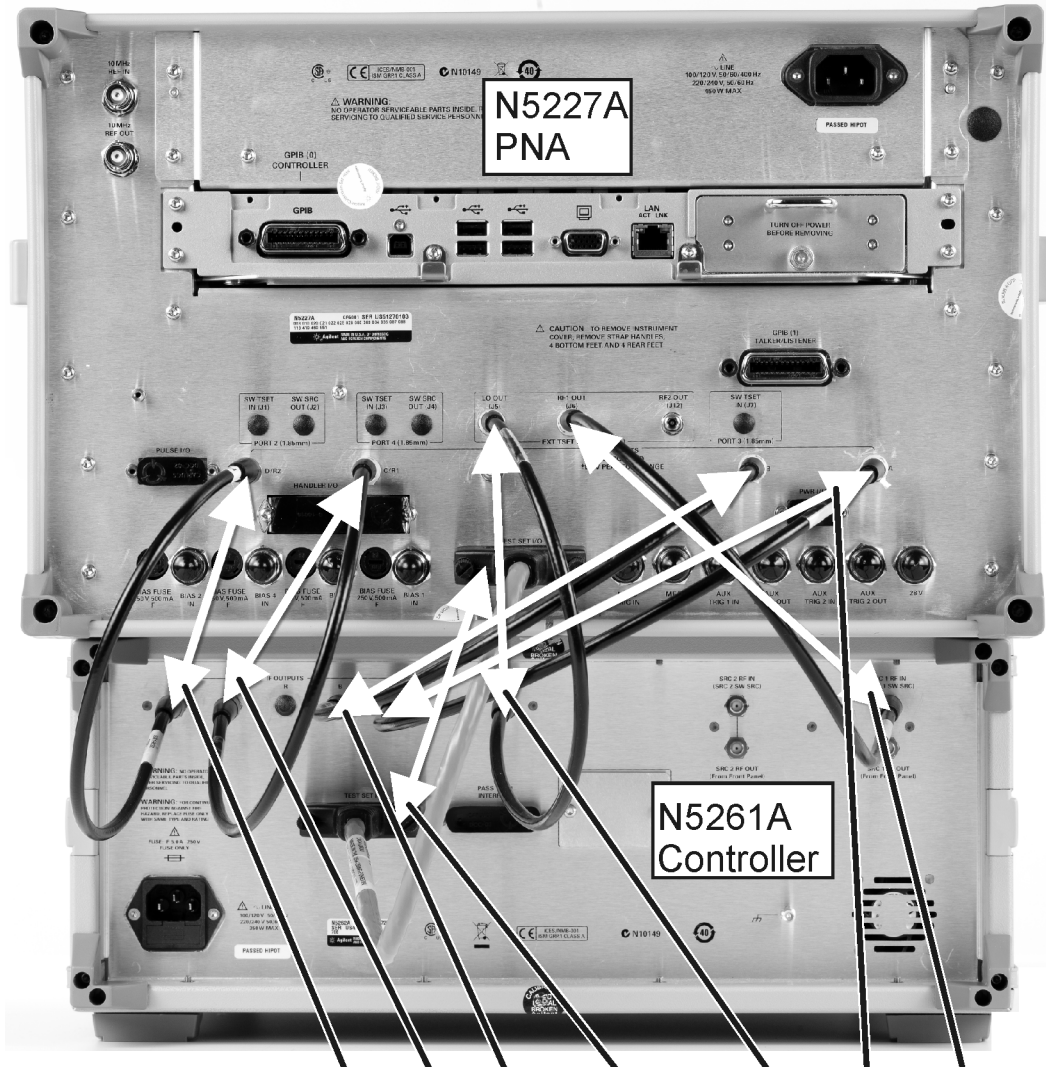
Figure 3-1 2-Port Model Rear Panel Cabling
