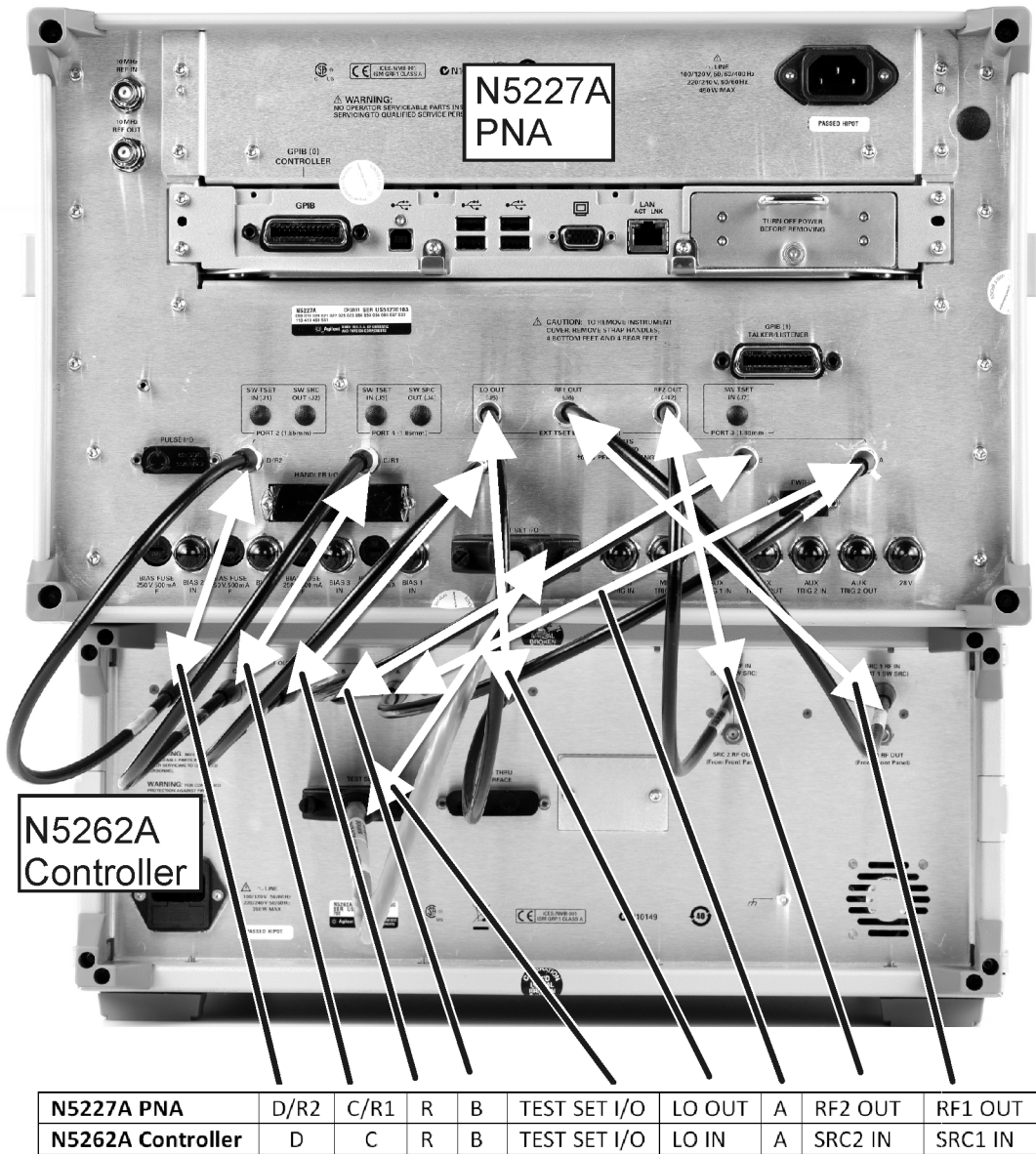
Figure 3-2 4-Port Model Rear Panel Cabling
