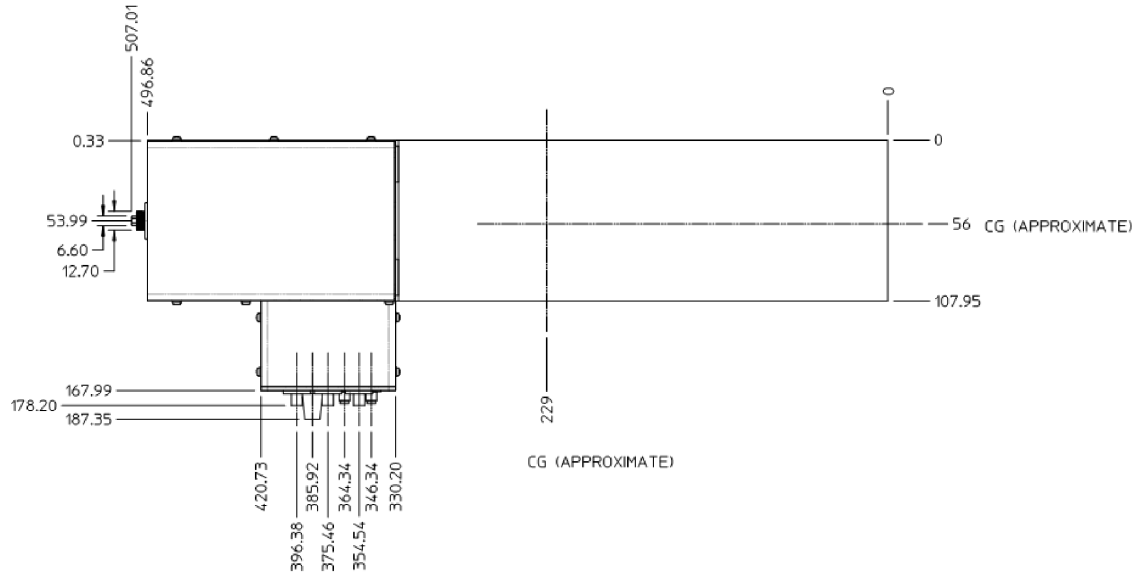
Figure 4-3. Test Head Module Dimensions for Mounting Left Test Head, Top View
