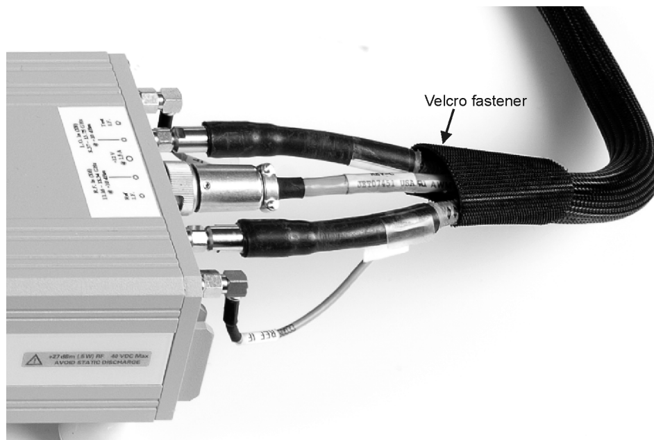
Figure 3-5 Details for Test Head Module Connections
